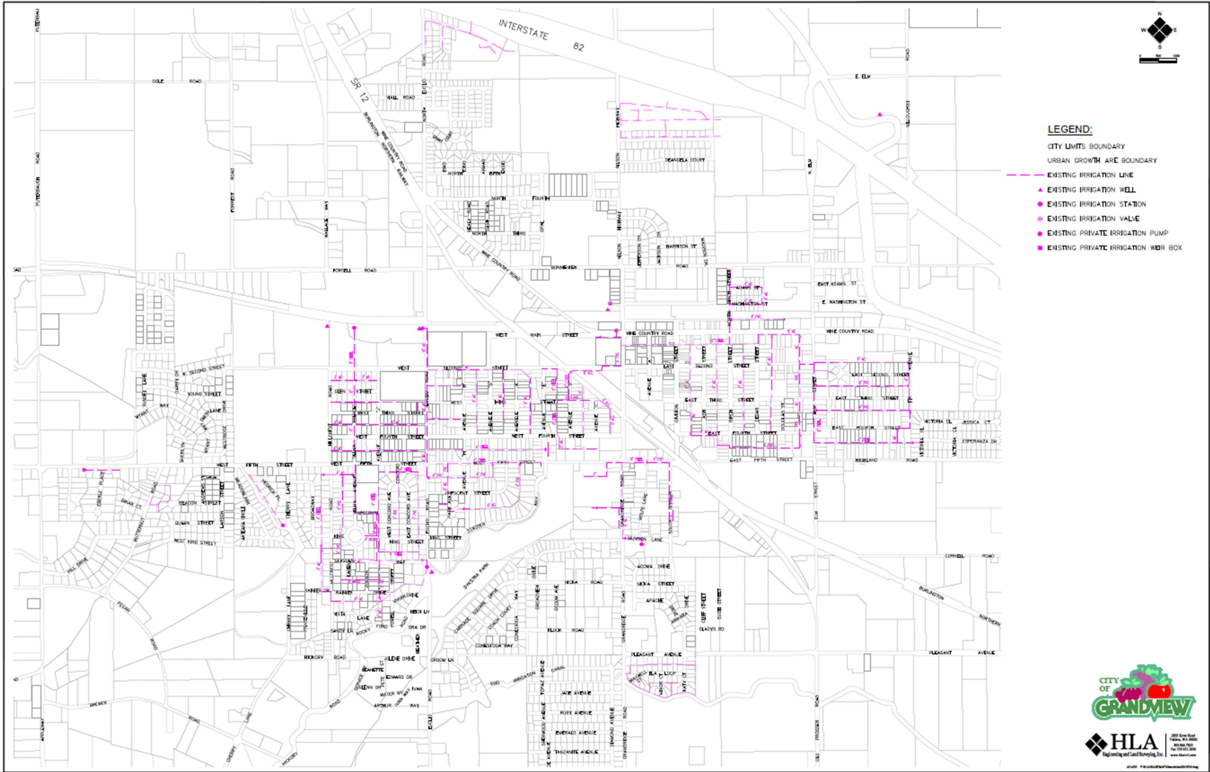
Figure 3-1 Irrigation Facilities
