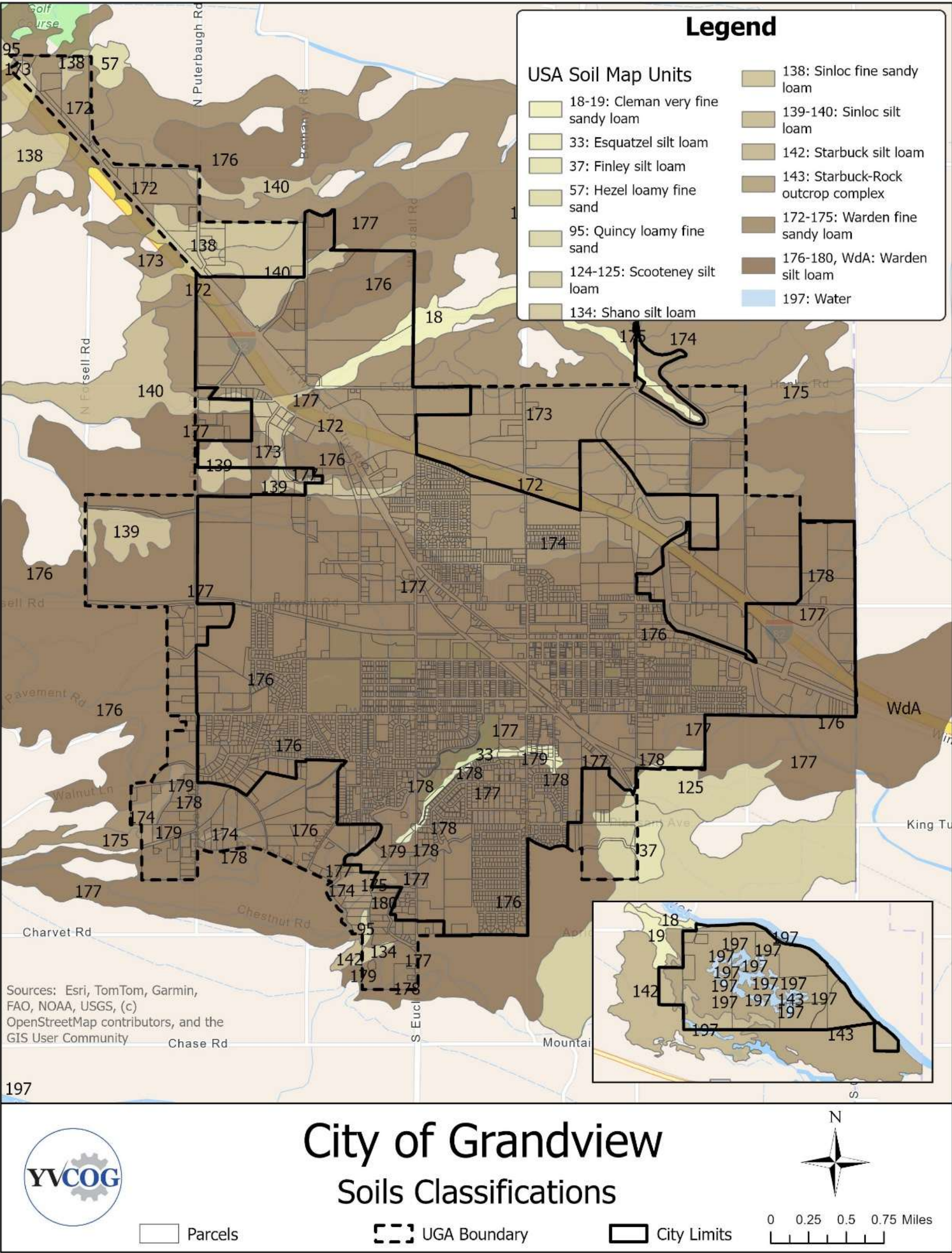
Figure 1.1 Soil Types in the city of Grandview and UGA
