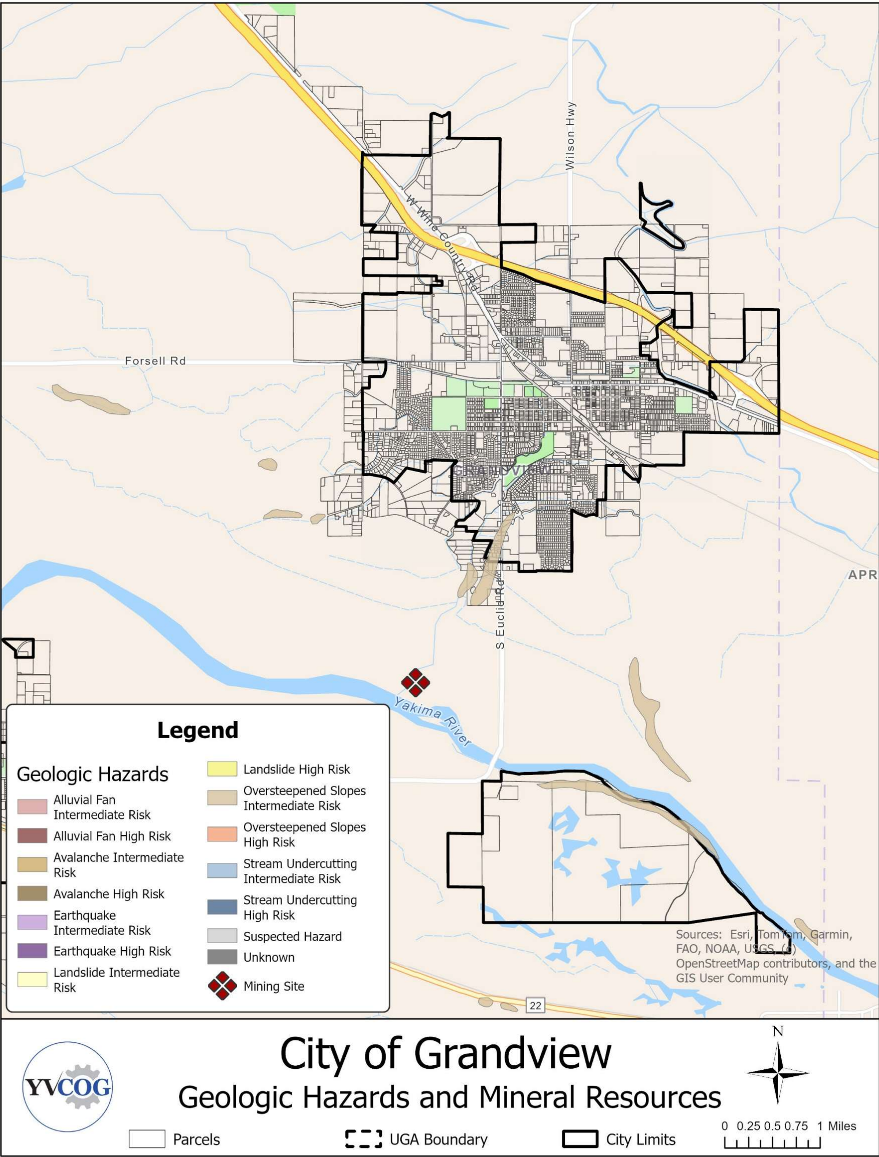
Figure 1-8. Geologic Hazard and Mineral Resource Areas, Grandview UGA
