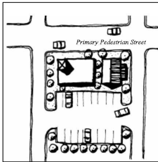
Driveways located off side streets
